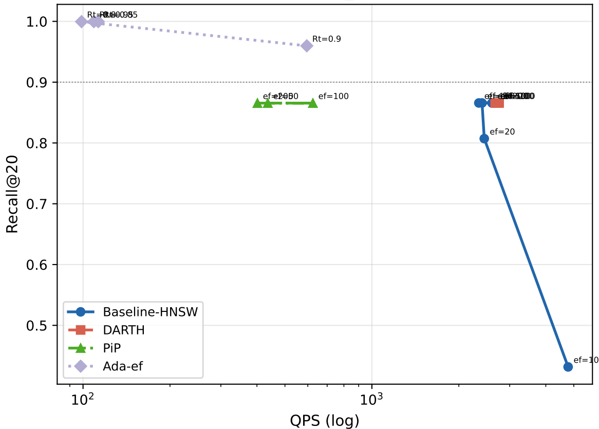
Recall@20-QPS — msmarco_text (M=16, efC=200)
