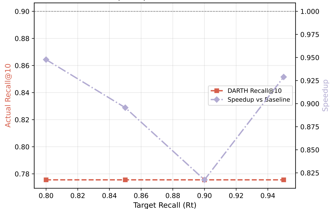
DARTH: Recall & Speedup vs Rt — sift128 (M=16, efC=200)
