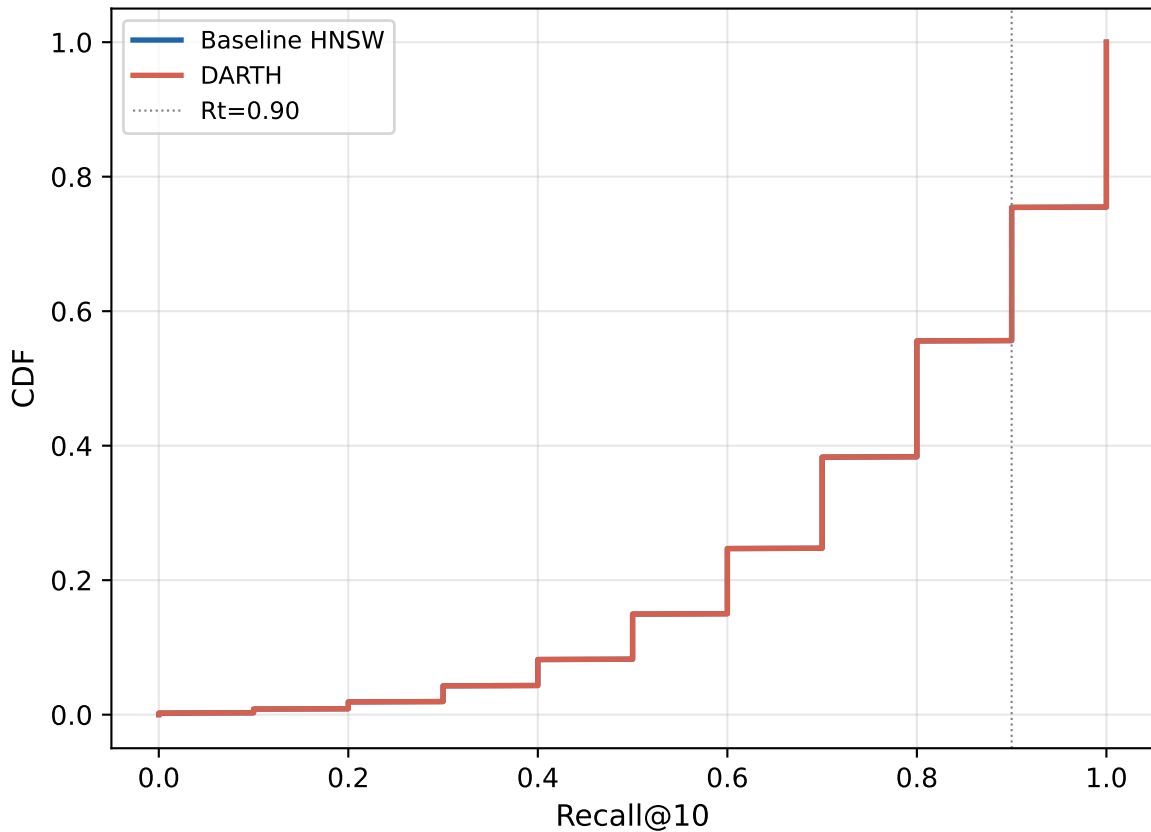
CDF of per-query Recall@10 — sift128
