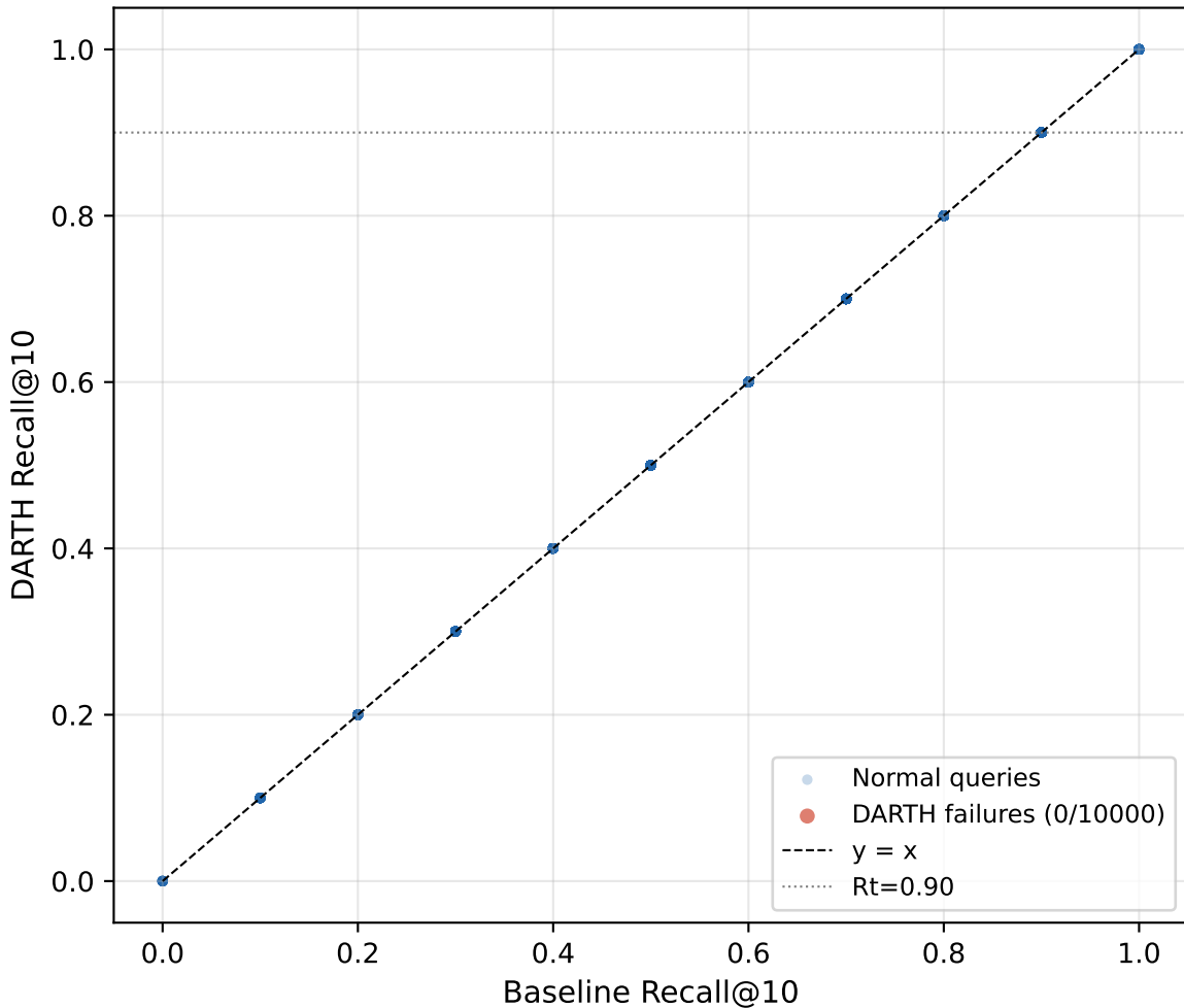
Per-query recall: Baseline vs DARTH — sift128
