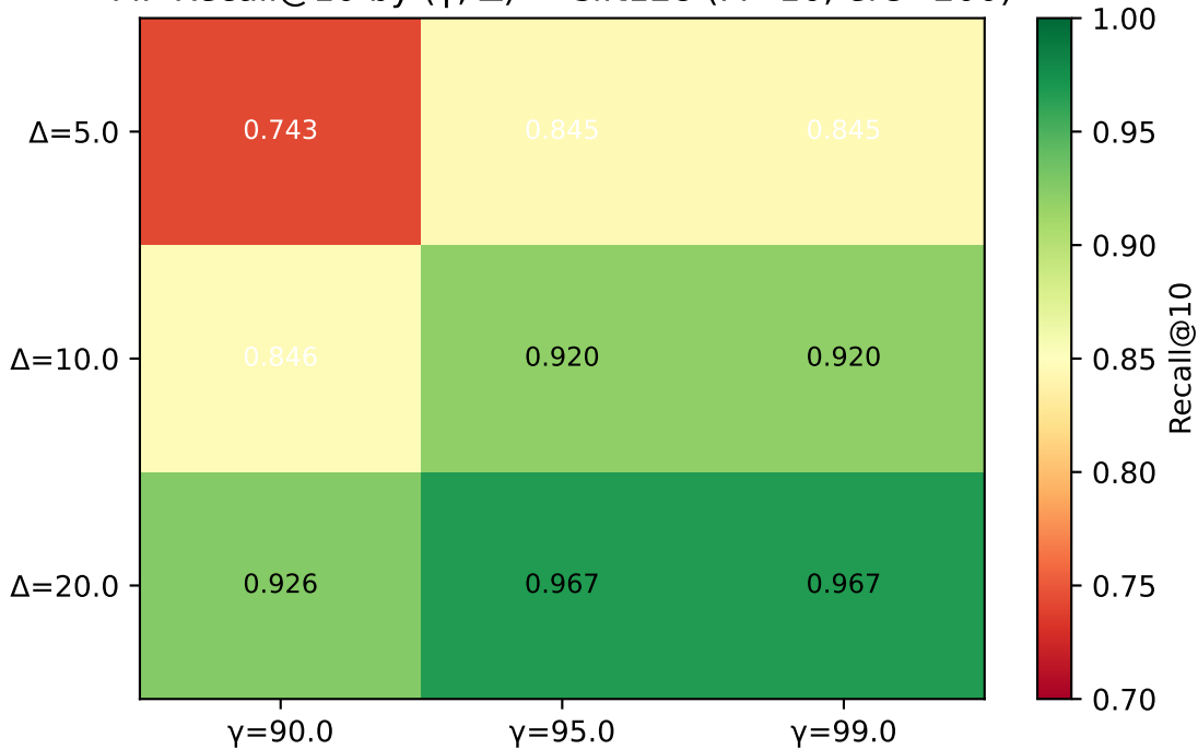
PiP Recall@10 by ( \gamma , \Delta ) — sift128 (M=16, efC=200)
