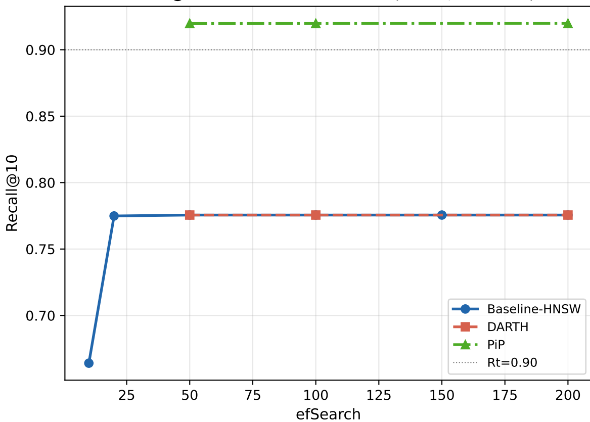
Recall@10 vs efSearch — sift128 (M=16, efC=200)
