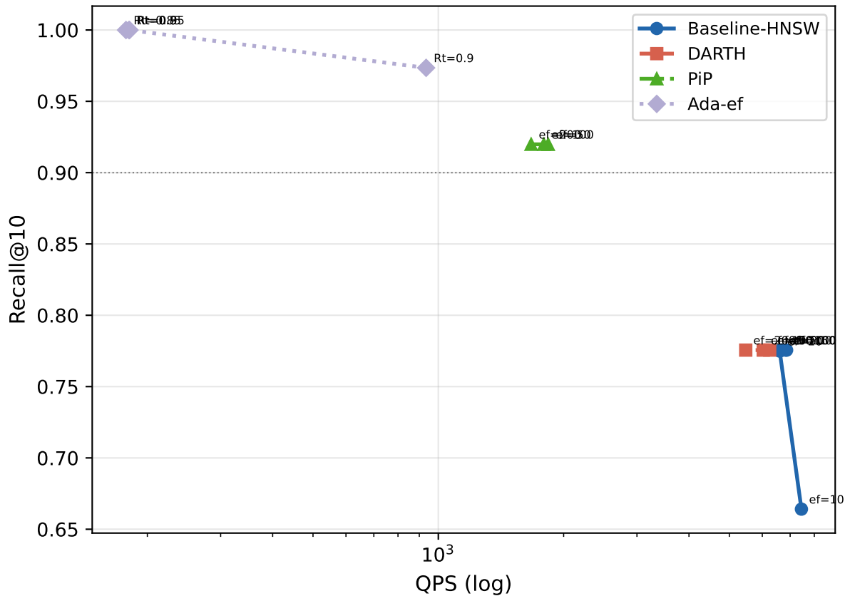
Recall@10-QPS — sift128 (M=16, efC=200)
