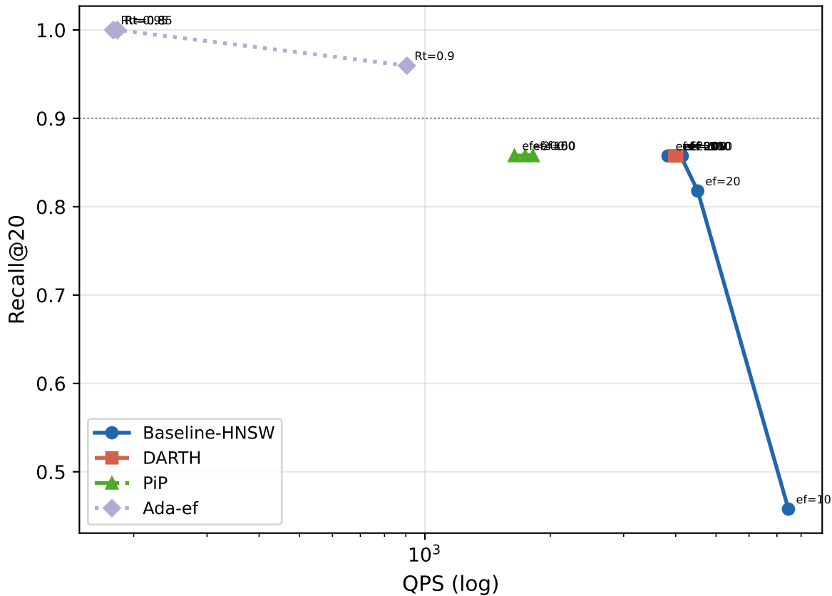
Recall@20-QPS — sift128 (M=16, efC=200)
