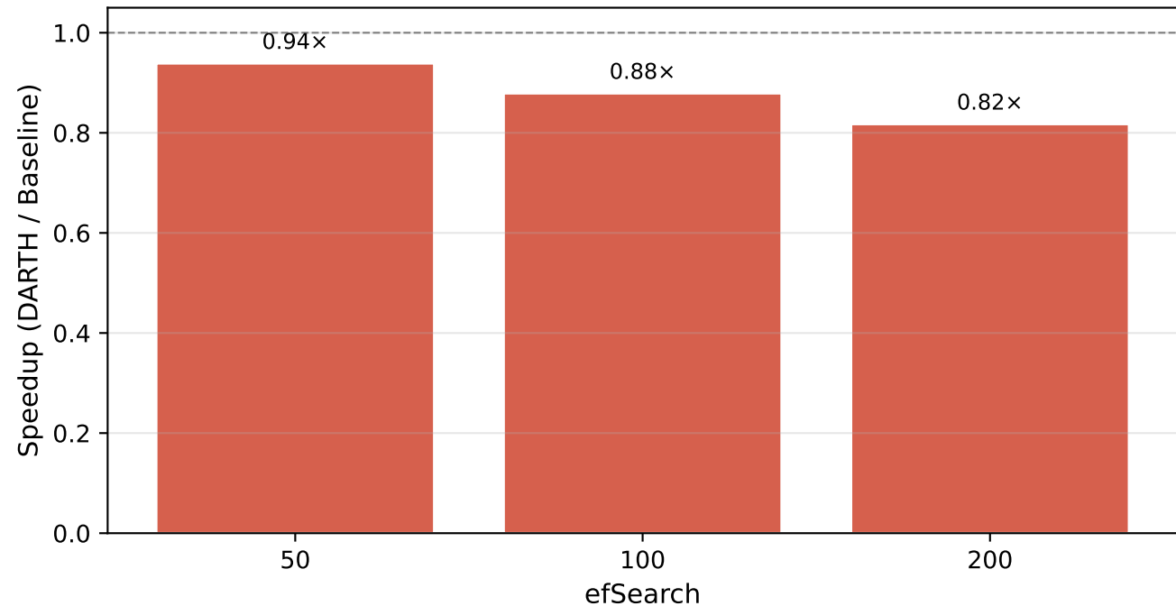
DARTH Speedup at R_t=0.90 — sift128 ( M=16 , efC=200 , k=10 )
