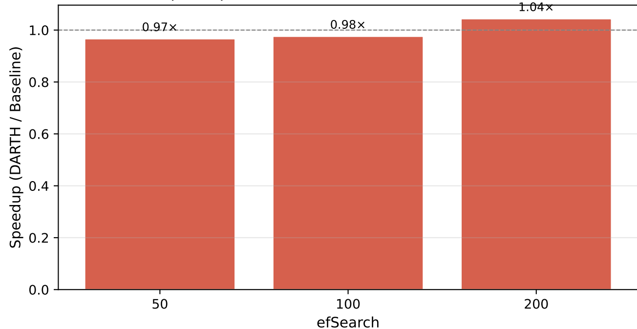
DARTH Speedup at Rt=0.90 — sift128 (M=16, efC=200, k=20)
