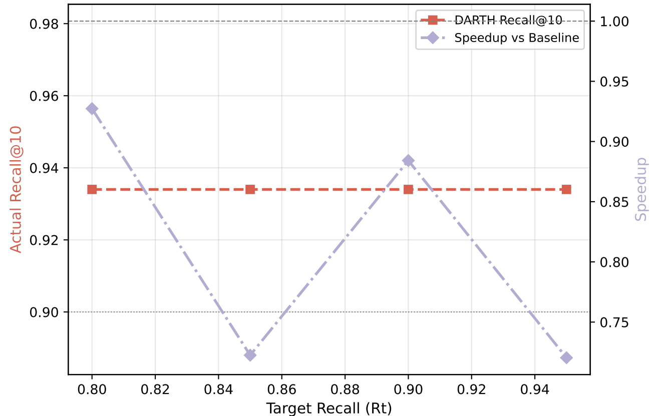
DARTH: Recall & Speedup vs Rt — siftsmall (M=16, efC=200)
