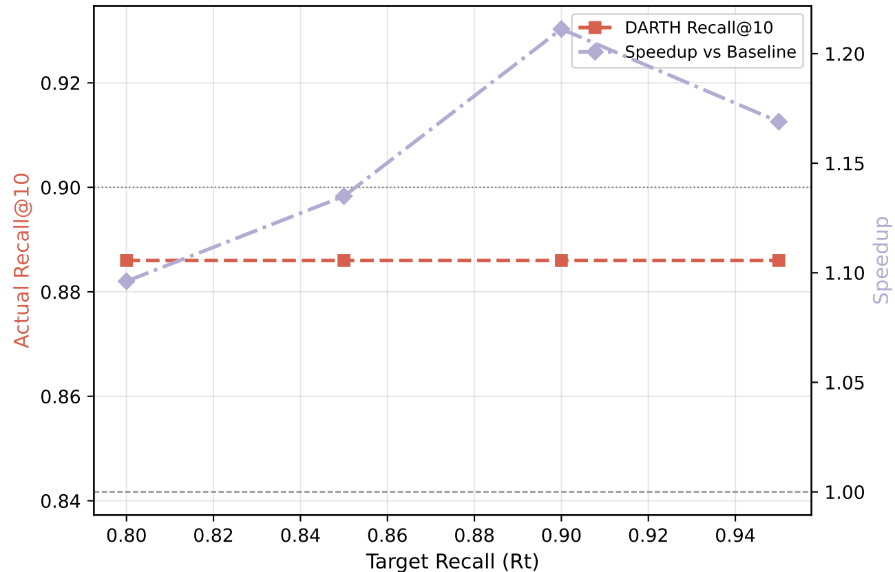
DARTH: Recall & Speedup vs Rt — siftsmall (M=8, efC=128)
