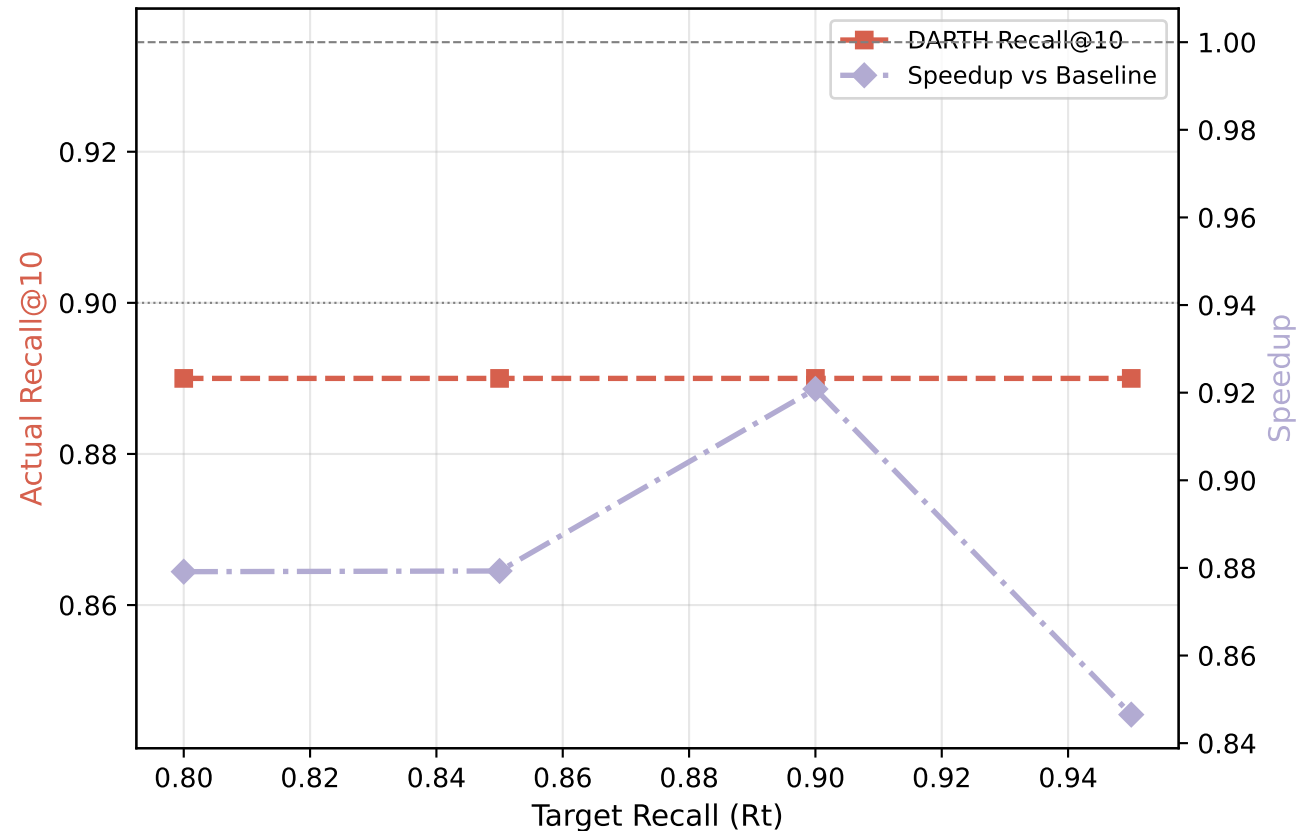
DARTH: Recall & Speedup vs Rt — siftsmall (M=8, efC=200)
