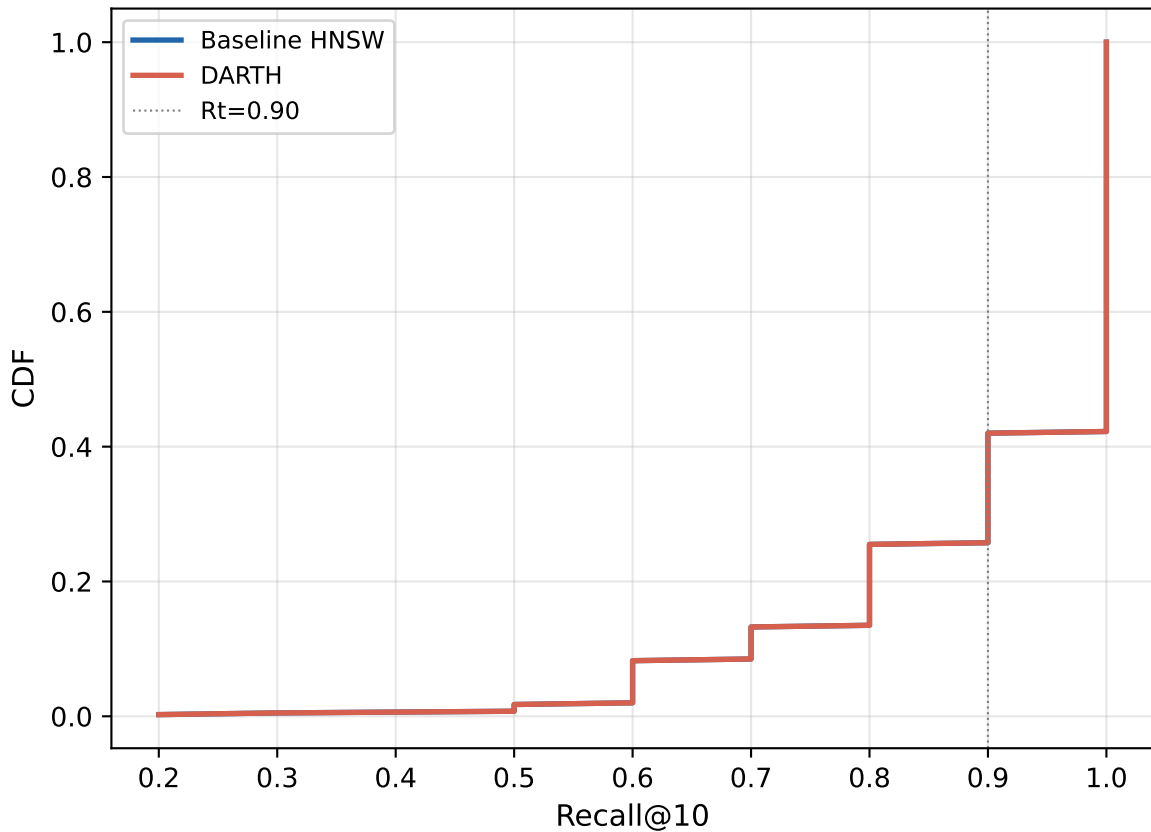
CDF of per-query Recall@10 — siftsmall
