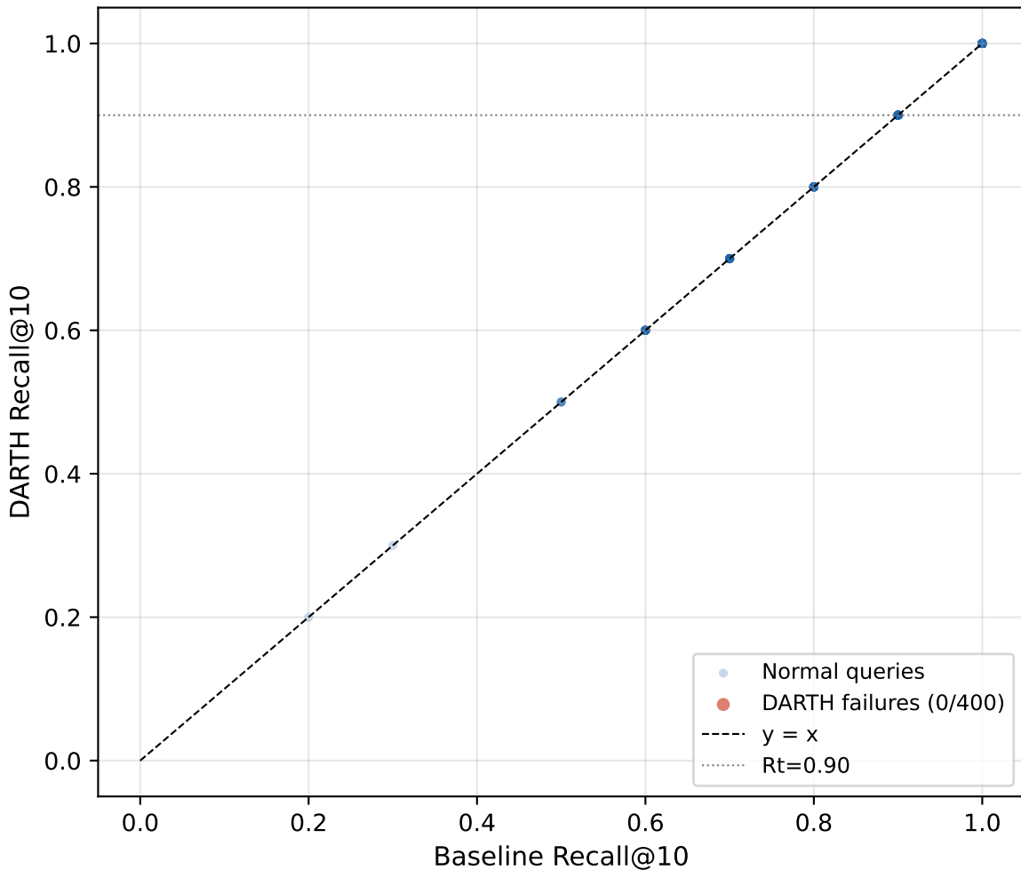
Per-query recall: Baseline vs DARTH — siftsmall
