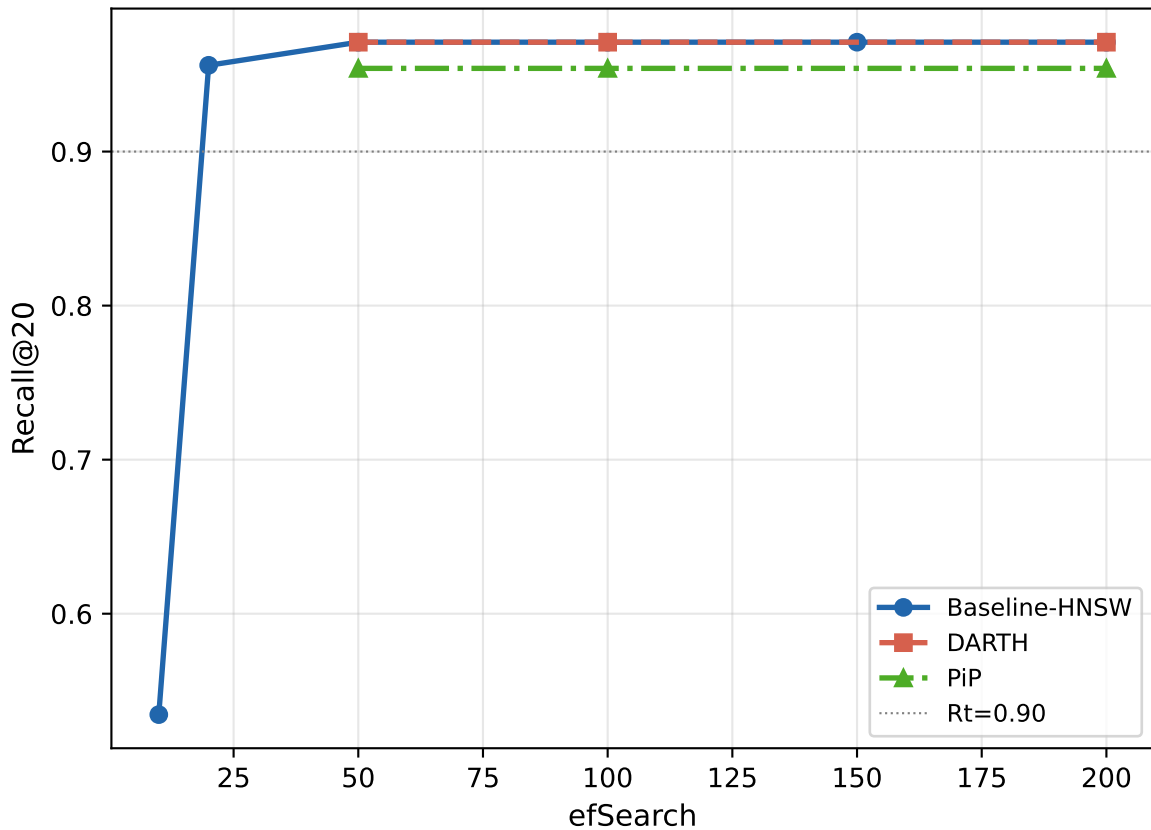
Recall@20 vs efSearch — siftsmall (M=16, efC=128)
