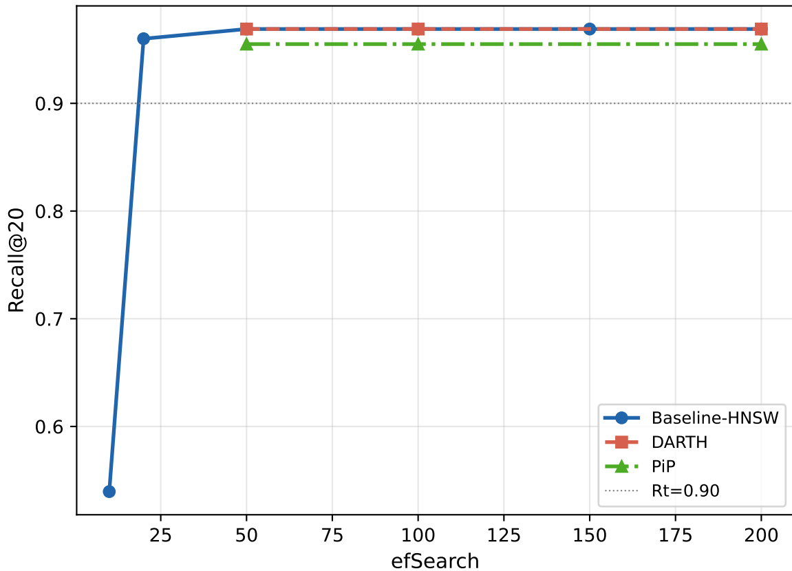
Recall@20 vs efSearch — siftsmall (M=16, efC=200)
