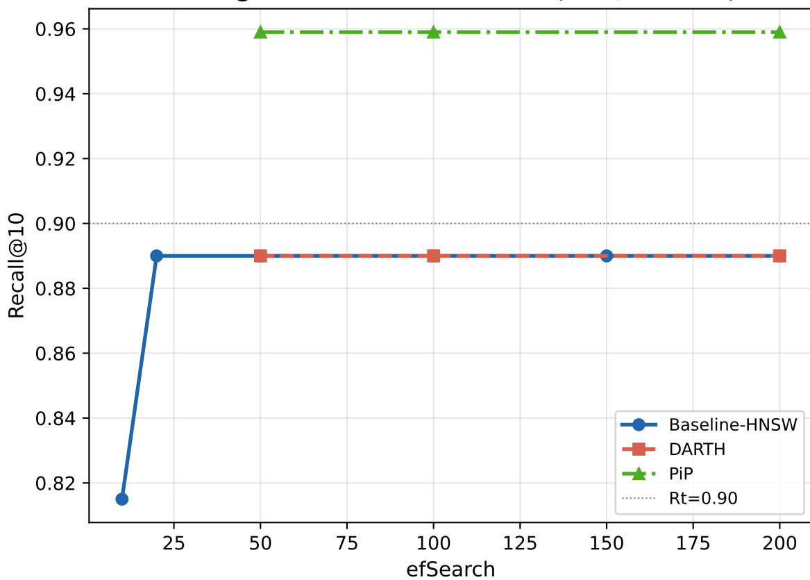
Recall@10 vs efSearch — siftsmall (M=8, efC=200)
