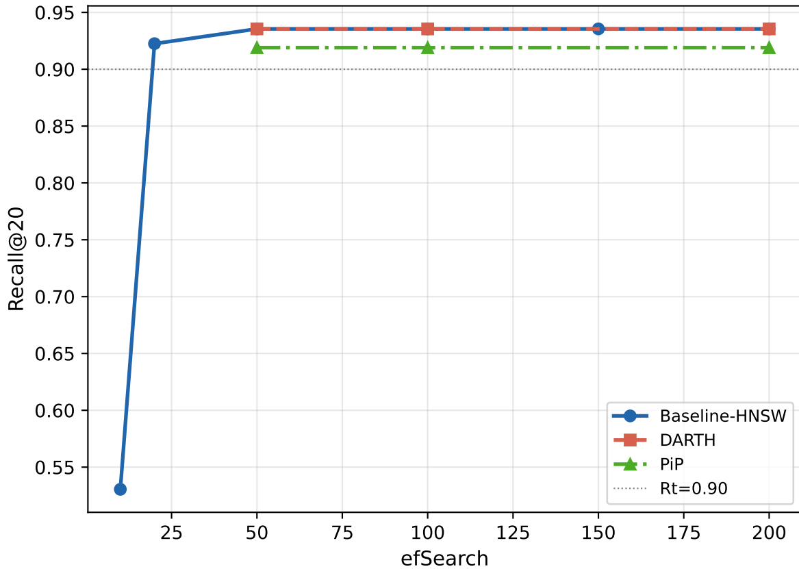
Recall@20 vs efSearch — siftsmall (M=8, efC=200)
