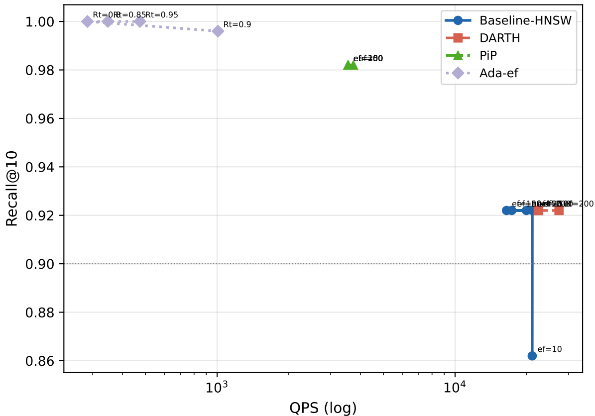
Recall@10-QPS — siftsmall (M=16, efC=128)
