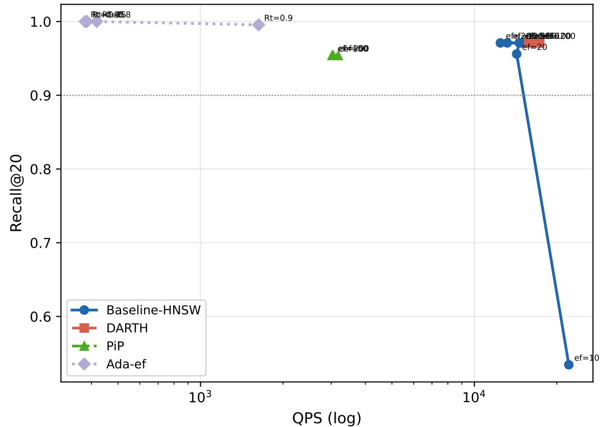
Recall@20-QPS — siftsmall (M=16, efC=128)
