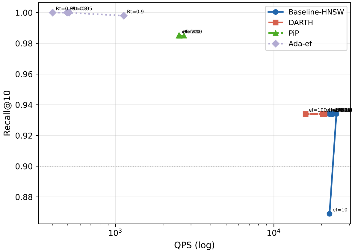
Recall@10-QPS — siftsmall (M=16, efC=200)
