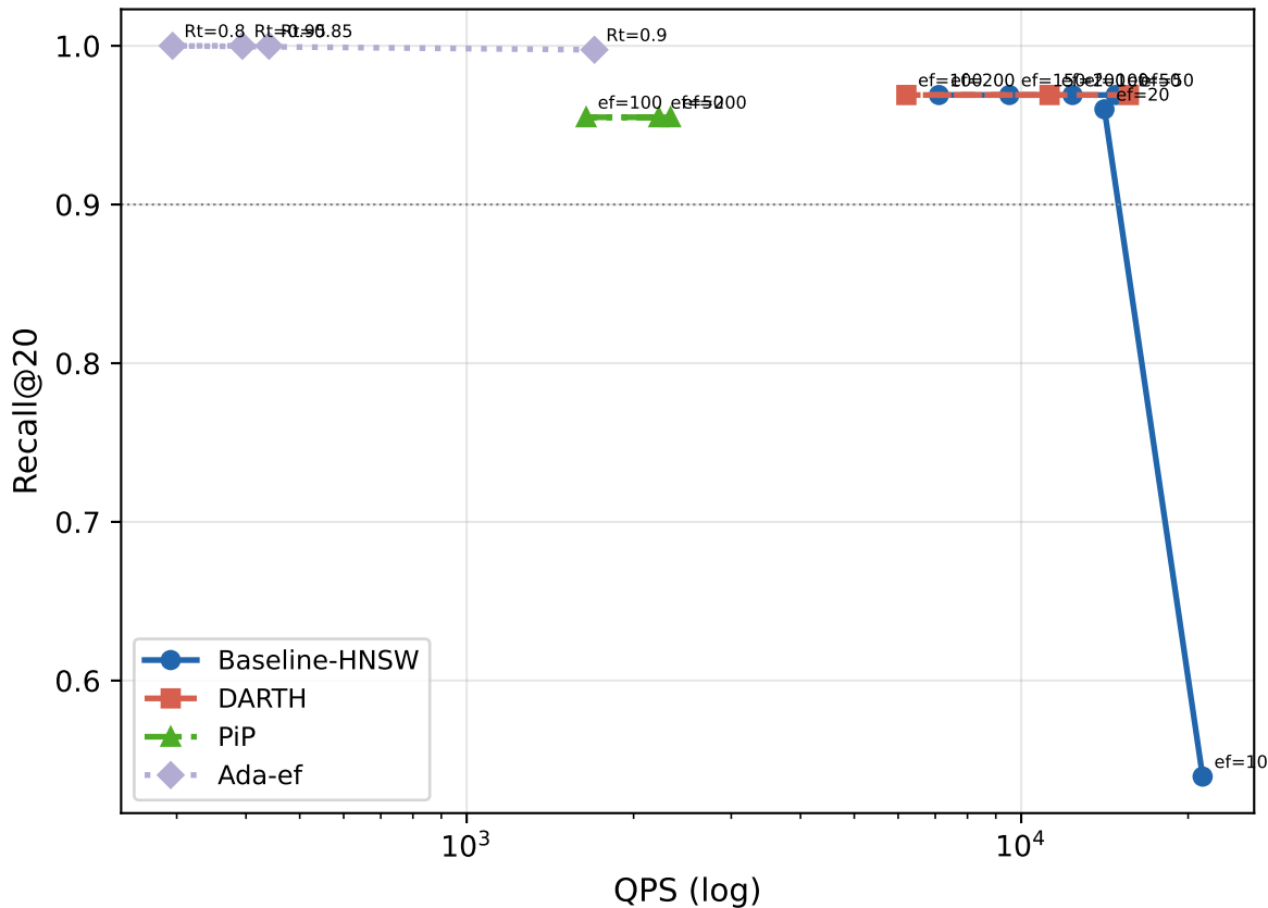
Recall@20-QPS — siftsmall (M=16, efC=200)
