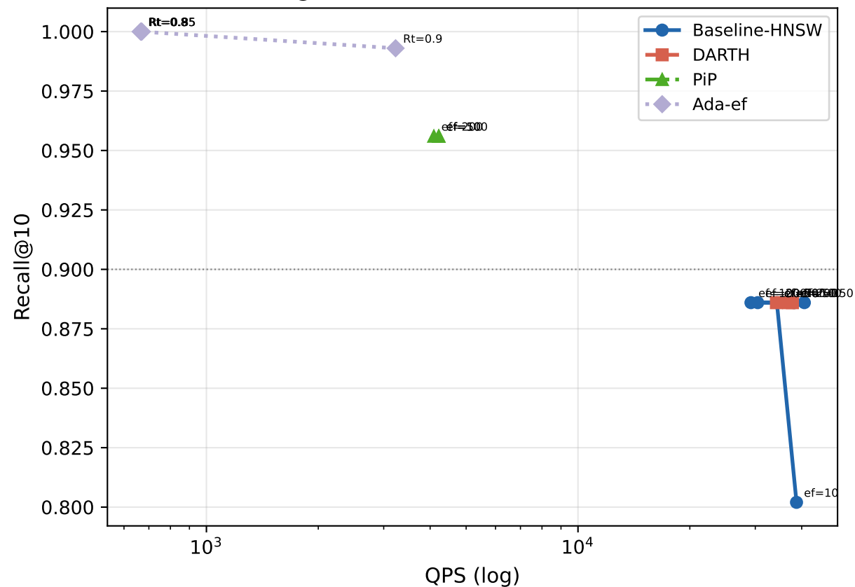
Recall@10-QPS — siftsmall (M=8, efC=128)
