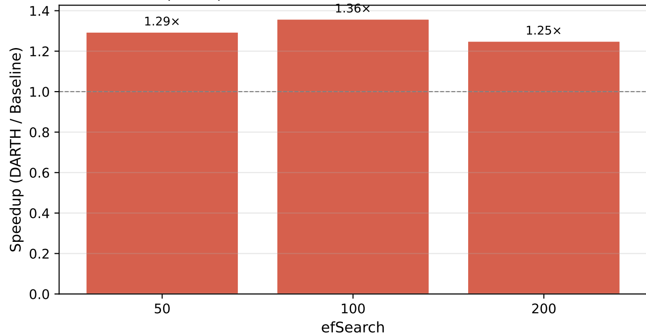
DARTH Speedup at Rt=0.90 — siftsmall (M=16, efC=128, k=10)
