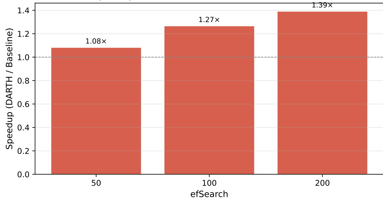
DARTH Speedup at Rt=0.90 — siftsmall (M=16, efC=128, k=20)
