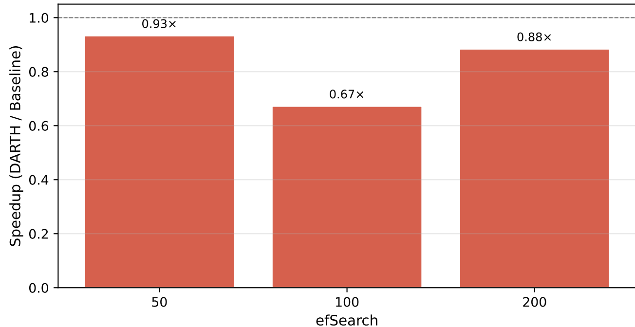
DARTH Speedup at R_t=0.90 — siftsmall ( M=16 , efC=200 , k=10 )
