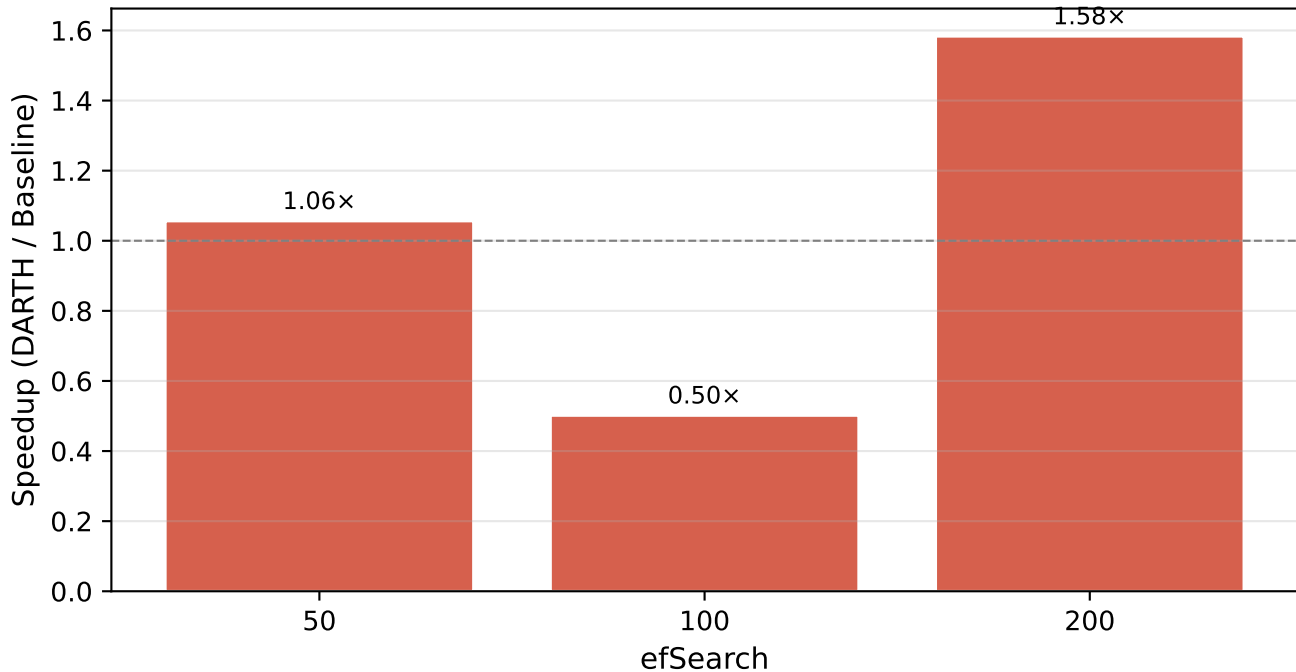
DARTH Speedup at Rt=0.90 — siftsmall (M=16, efC=200, k=20)
