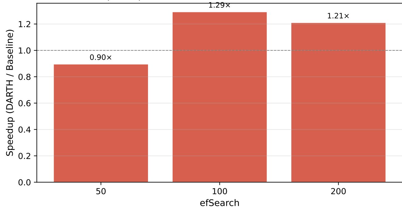
DARTH Speedup at Rt=0.90 — siftsmall (M=8, efC=128, k=10)
