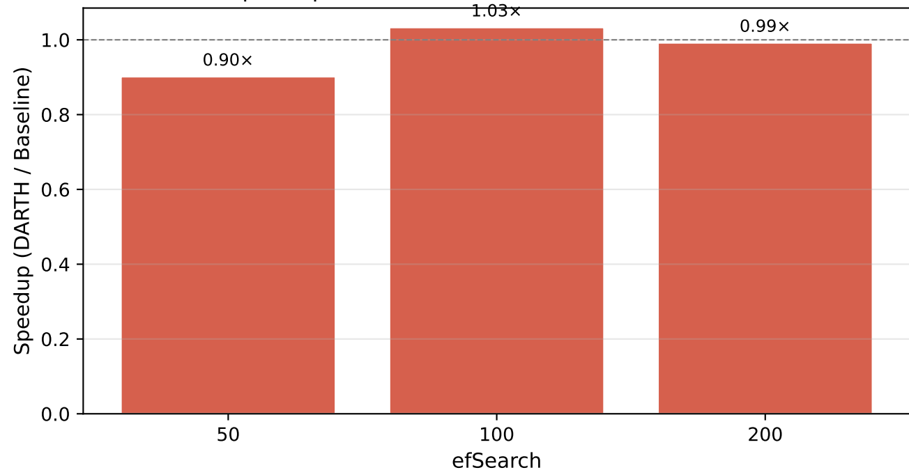
DARTH Speedup at Rt=0.90 — siftsmall (M=8, efC=128, k=20)
