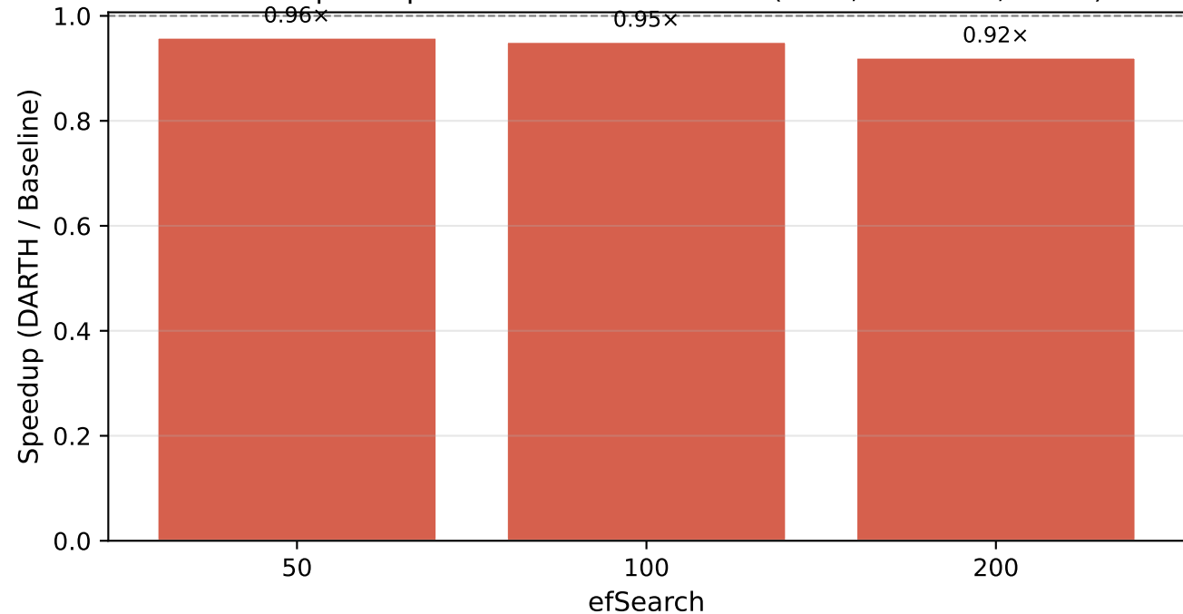
DARTH Speedup at Rt=0.90 — siftsmall (M=8, efC=200, k=10)
