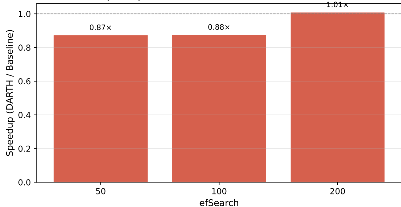
DARTH Speedup at R_t=0.90 — siftsmall ( M=8 , efC=200 , k=20 )
