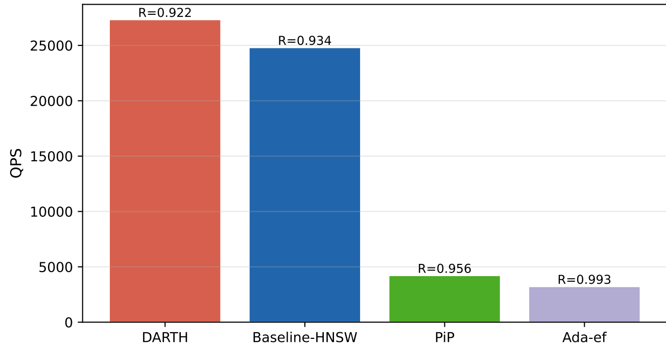
QPS at Recall@10 \geq 0.9 — siftsmall
