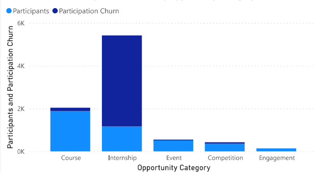
Participation vs Churn by Opportunity Category
