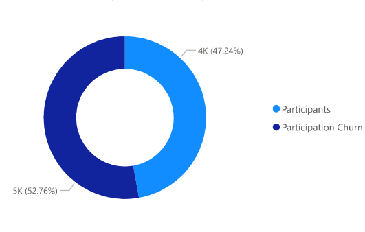
Participants and Participation Churn
