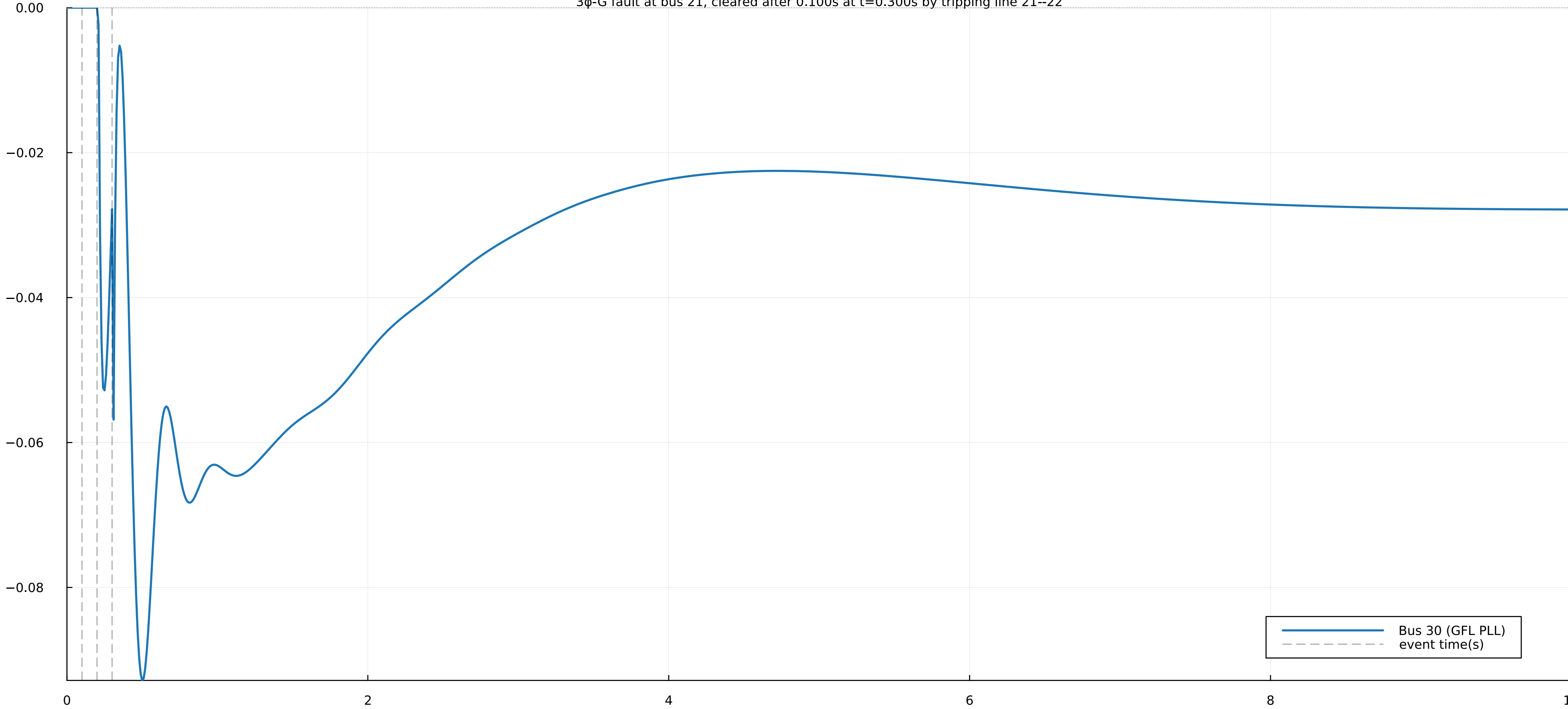
Frequency deviation at bus 30 3 \phi -G fault at bus 21, cleared after 0.100s at t=0.300s by tripping line 21--22
