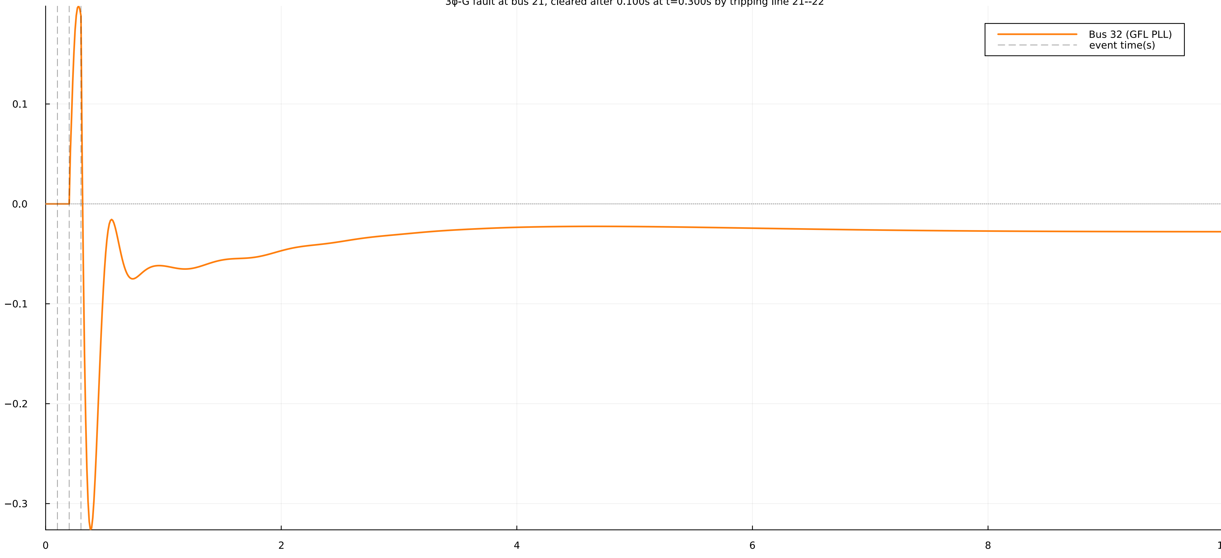
Frequency deviation at bus 32 3 \phi -G fault at bus 21, cleared after 0.100s at t=0.300s by tripping line 21--22
