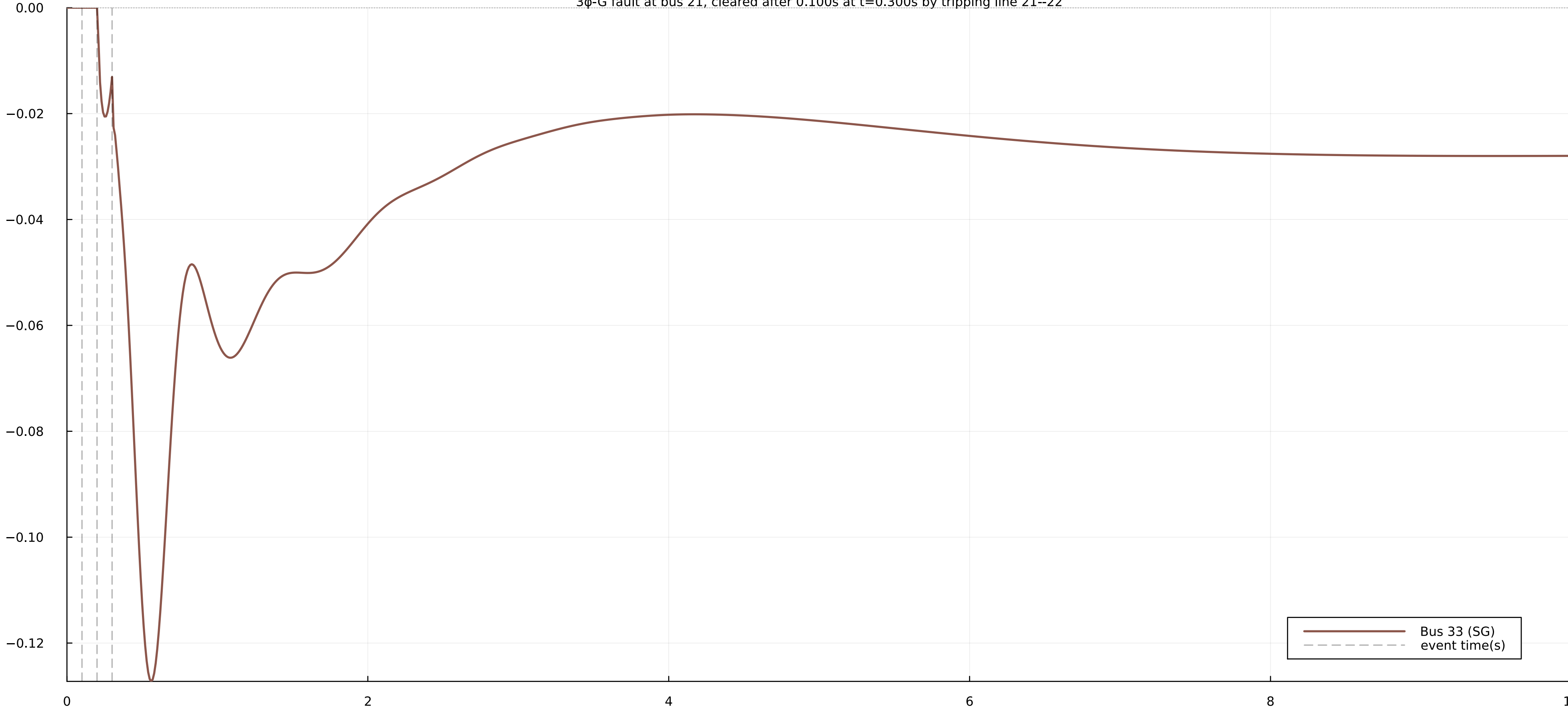
Frequency deviation at bus 33 3 \phi -G fault at bus 21, cleared after 0.100s at t=0.300s by tripping line 21--22
