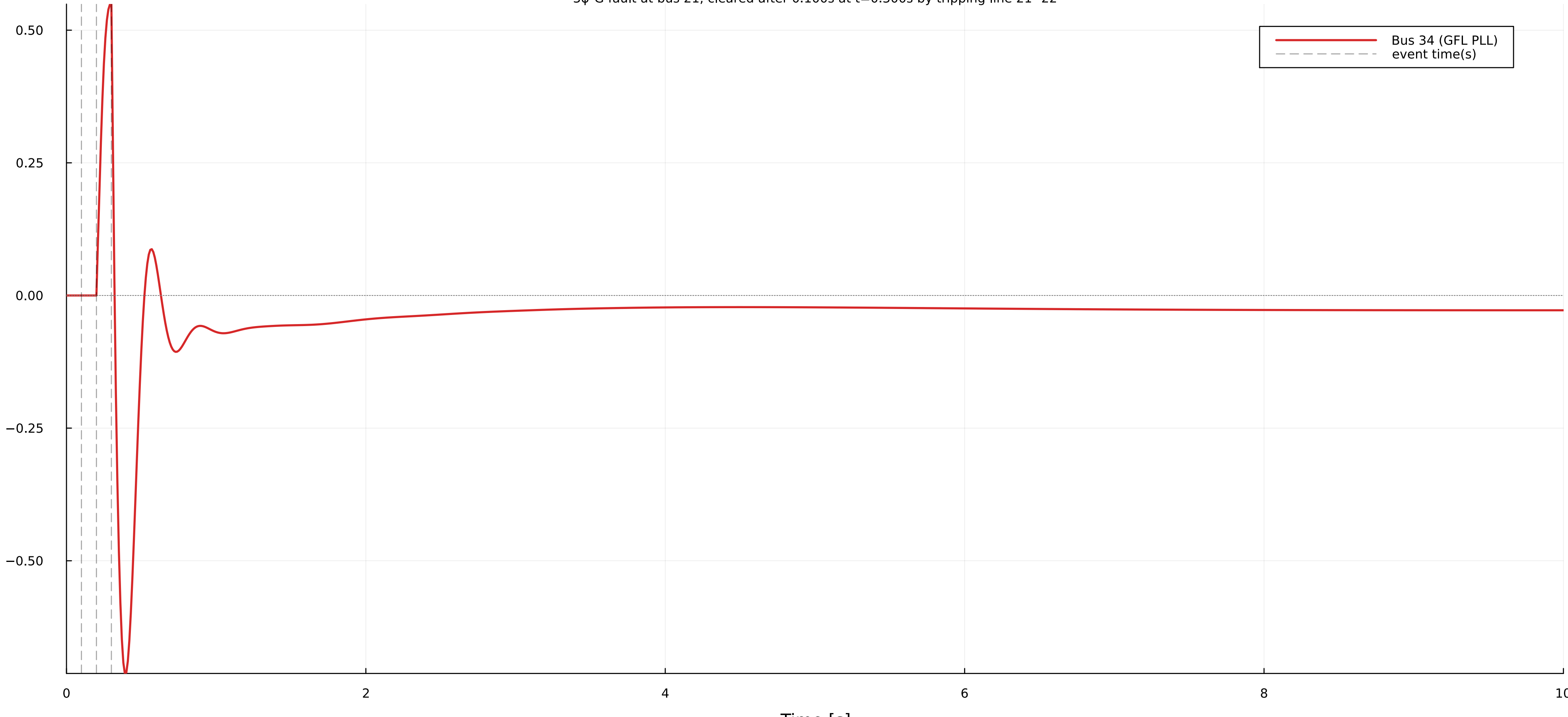
Frequency deviation at bus 34 3 \phi -G fault at bus 21, cleared after 0.100s at t=0.300s by tripping line 21--22
