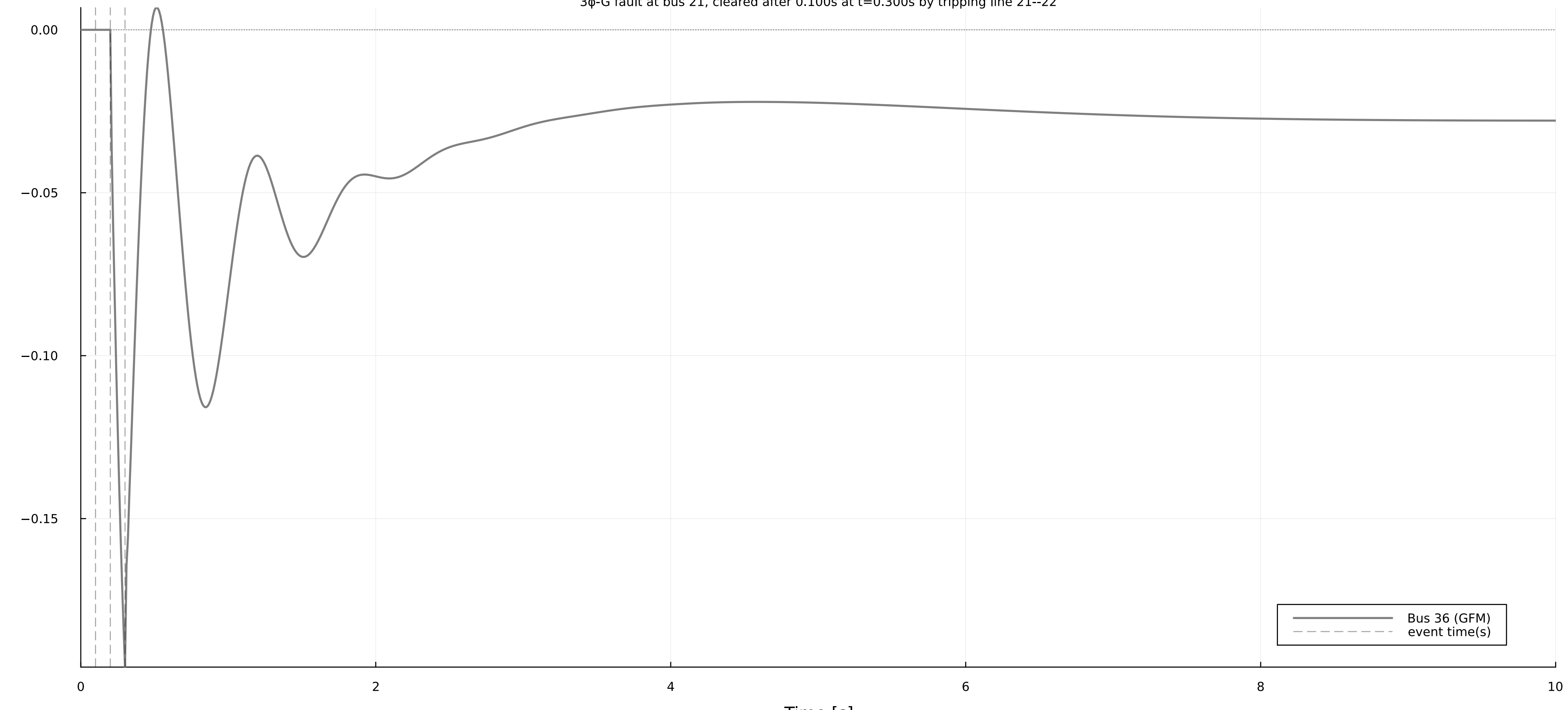
Frequency deviation at bus 36 3 \phi -G fault at bus 21, cleared after 0.100s at t=0.300s by tripping line 21--22
