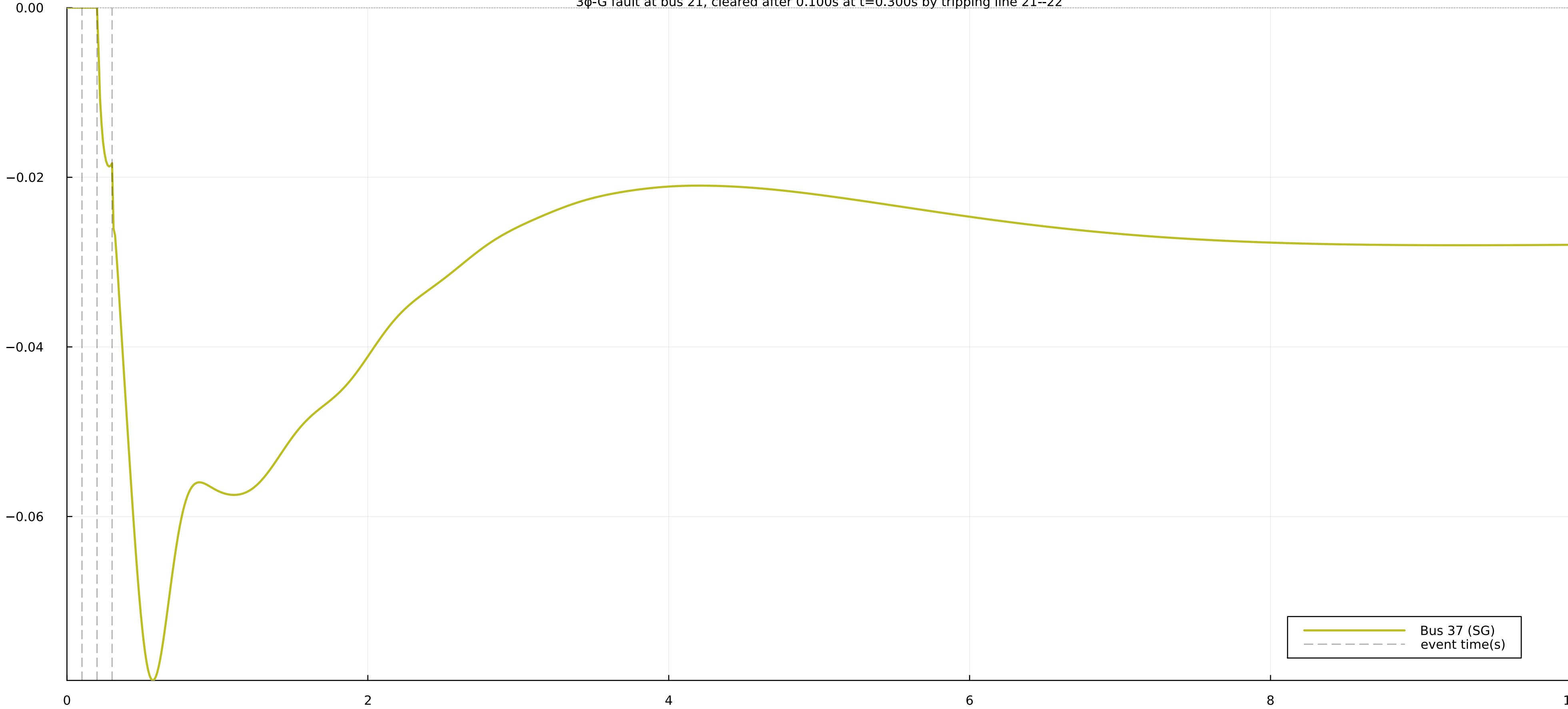
Frequency deviation at bus 37 3 \phi -G fault at bus 21, cleared after 0.100s at t=0.300s by tripping line 21--22
