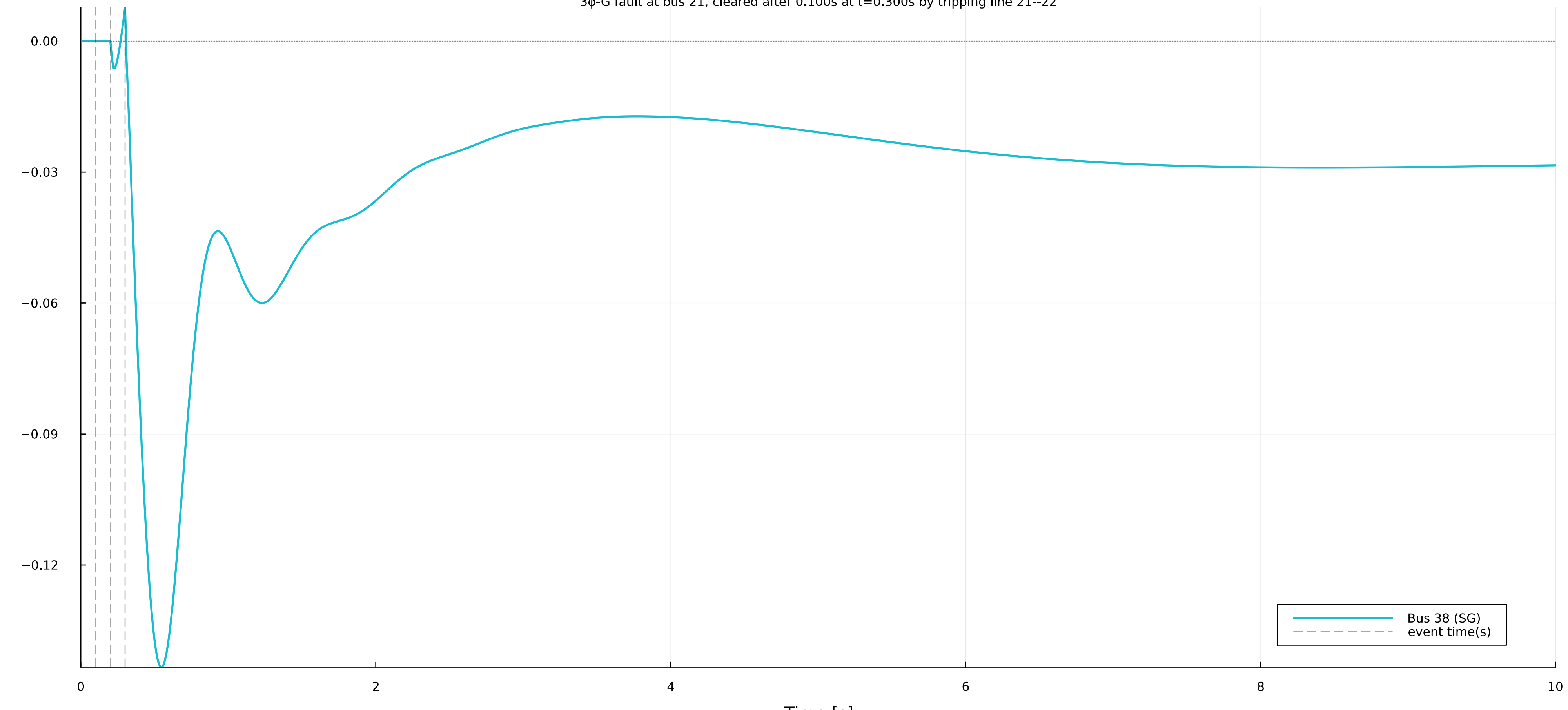
Frequency deviation at bus 38 3 \phi -G fault at bus 21, cleared after 0.100s at t=0.300s by tripping line 21--22
