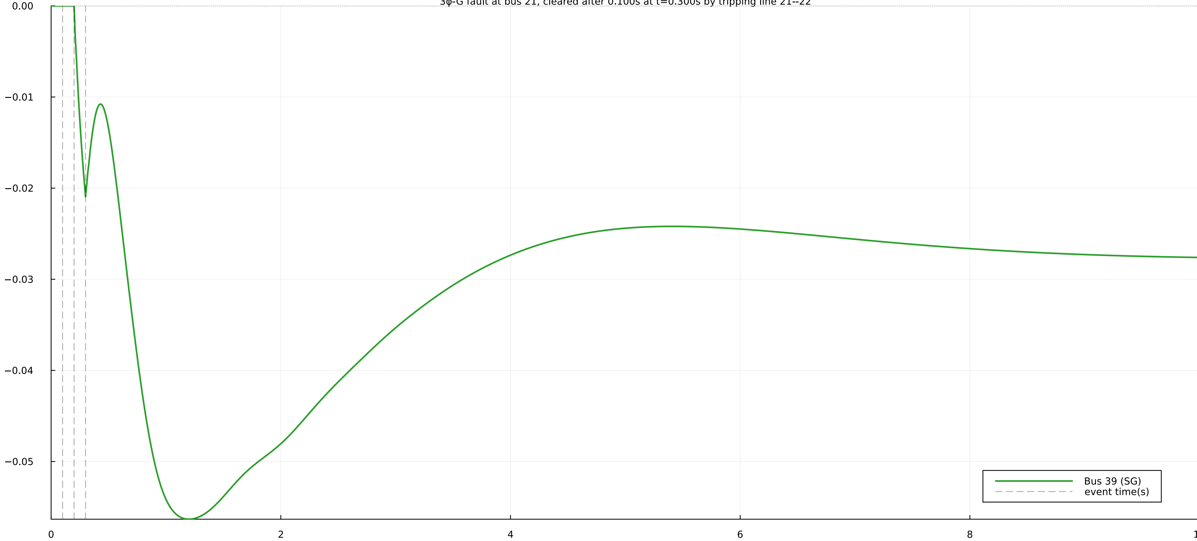
Frequency deviation at bus 39 3 \phi -G fault at bus 21, cleared after 0.100s at t=0.300s by tripping line 21--22
