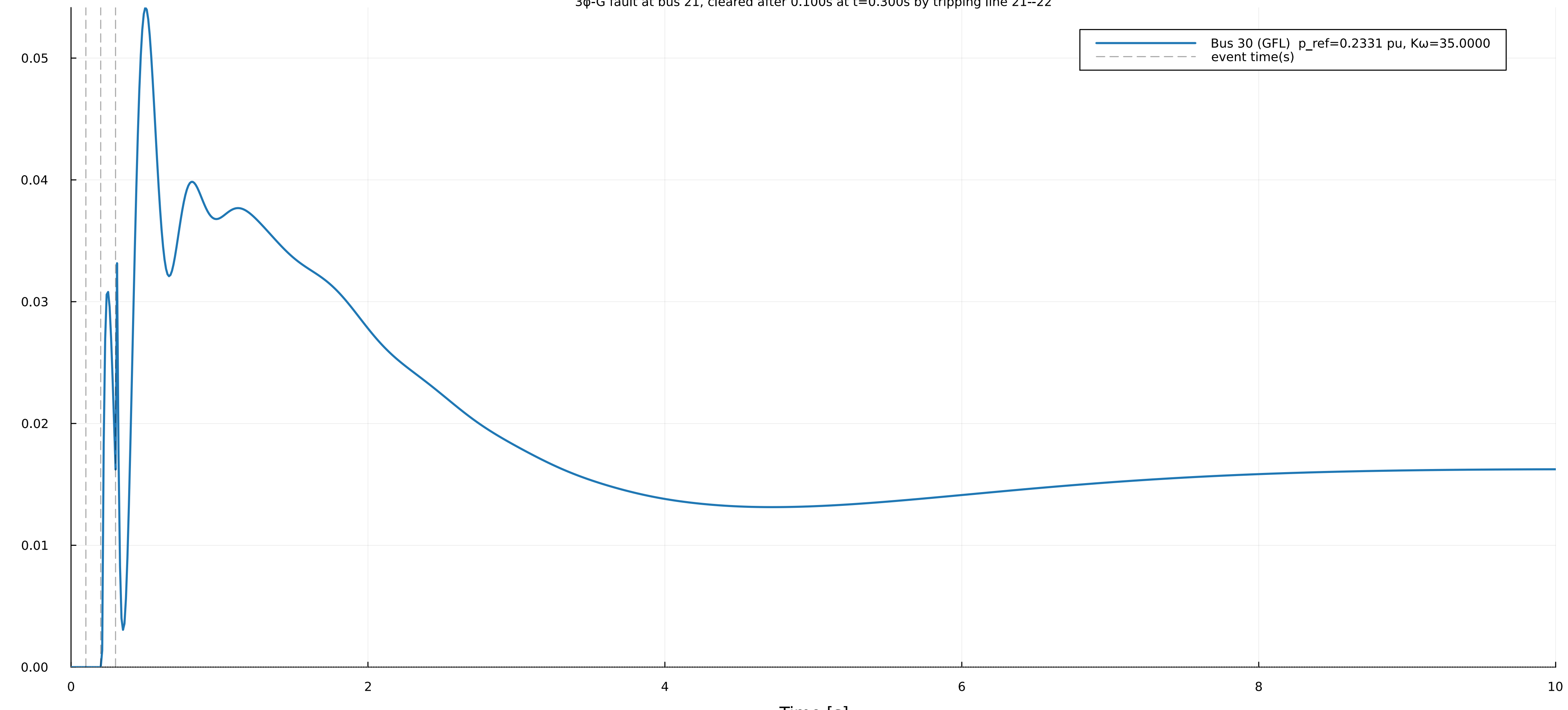
GFL effective P-ref deviation at bus 30 3φ-G fault at bus 21, cleared after 0.100s at t=0.300s by tripping line 21--22
