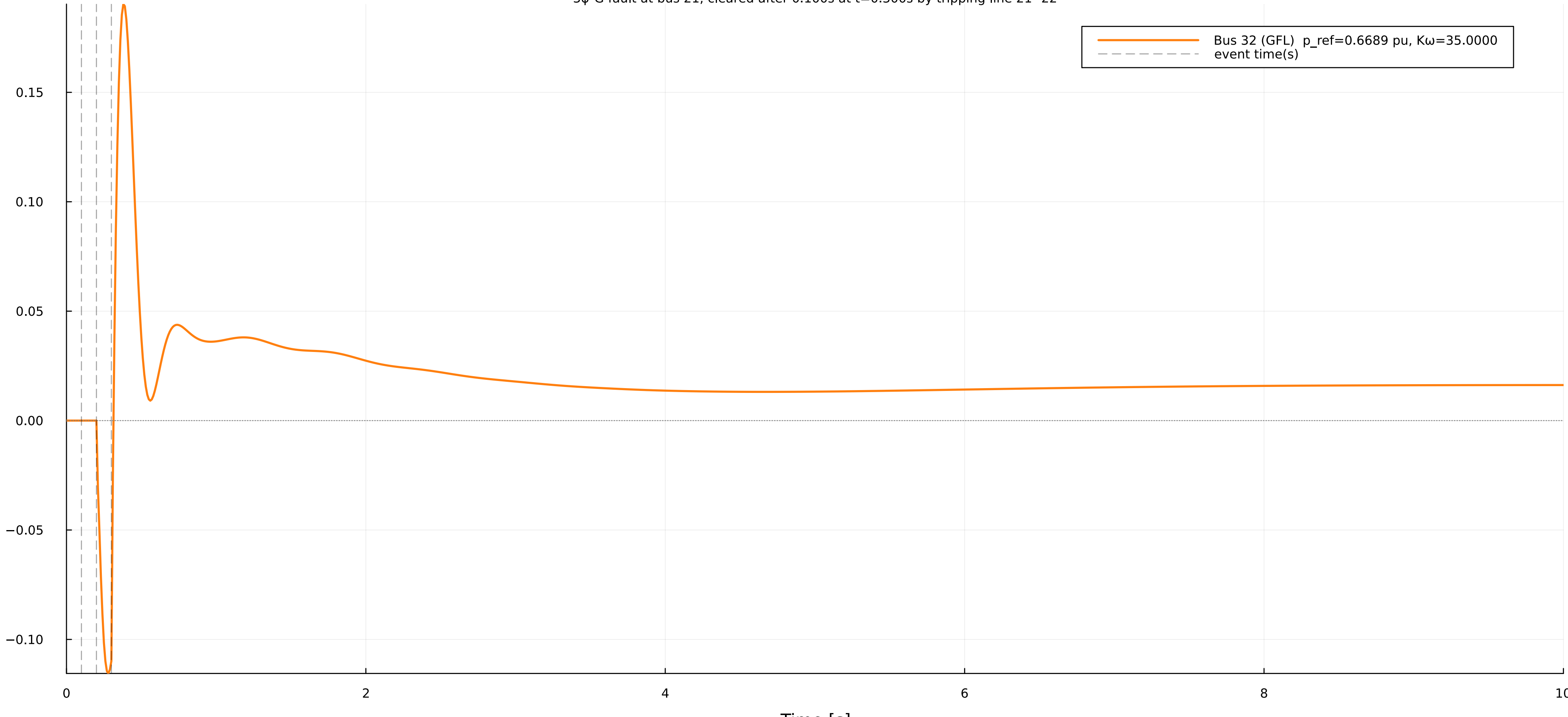
GFL effective P-ref deviation at bus 32 3 \phi -G fault at bus 21, cleared after 0.100s at t=0.300s by tripping line 21--22
