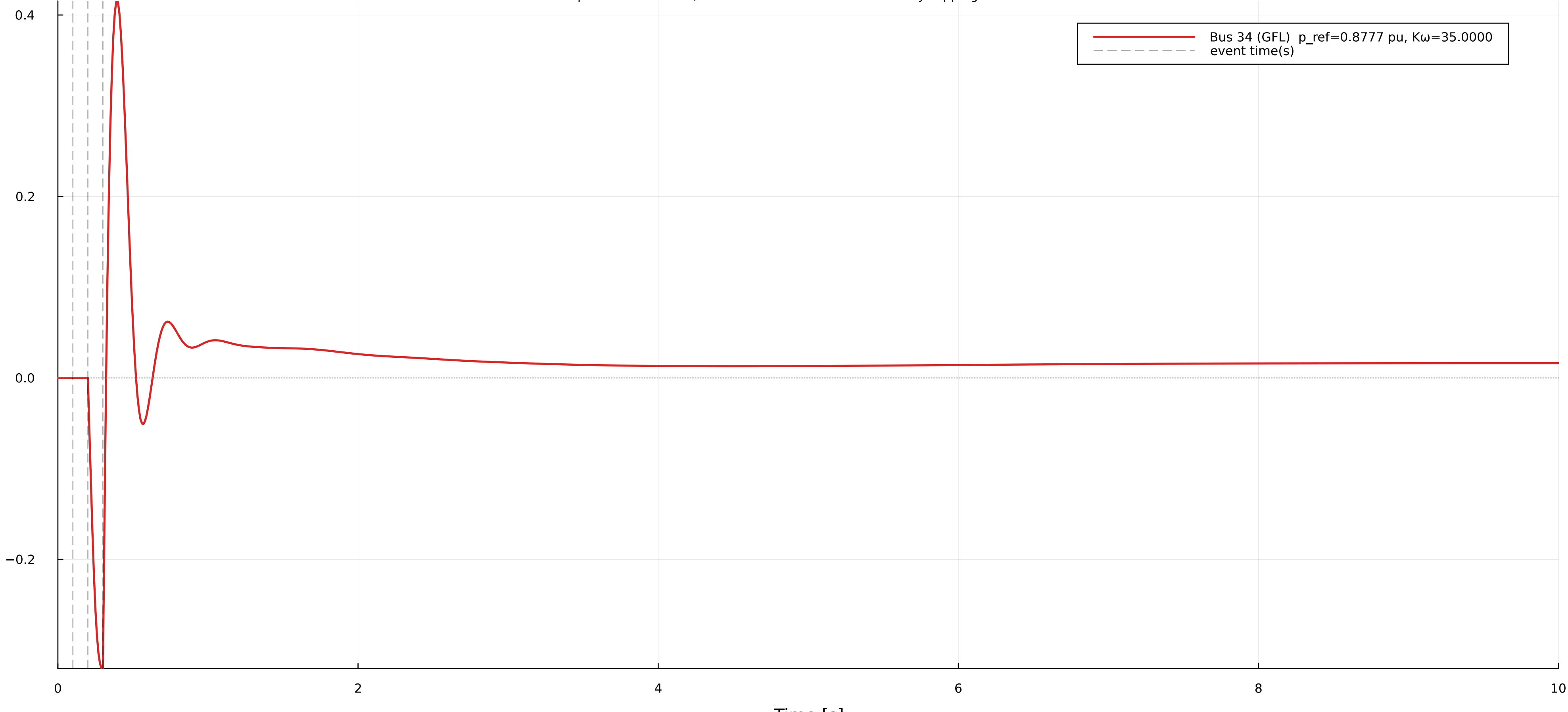
GFL effective P-ref deviation at bus 34 3φ-G fault at bus 21, cleared after 0.100s at t=0.300s by tripping line 21--22
