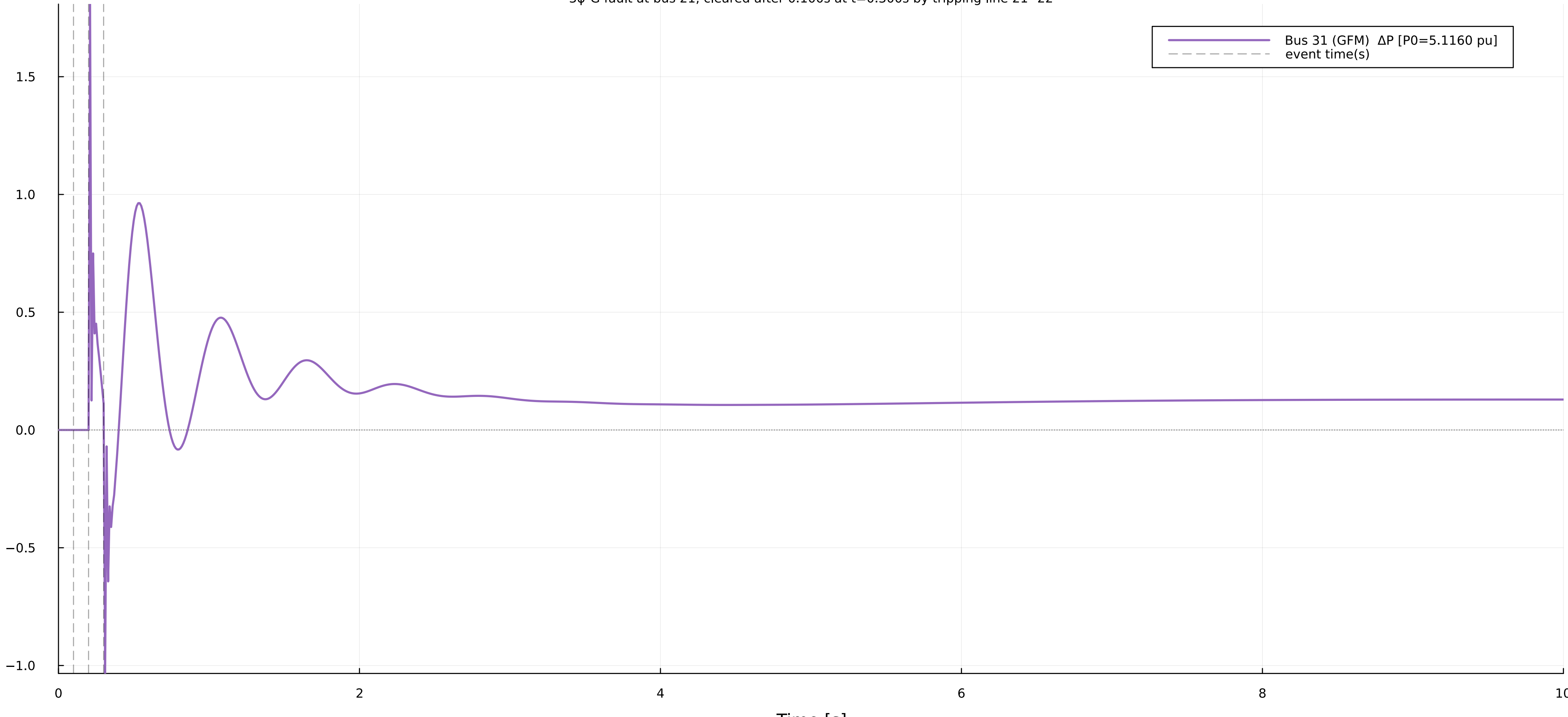
GFM active-power deviation at bus 31 3φ-G fault at bus 21, cleared after 0.100s at t=0.300s by tripping line 21--22
