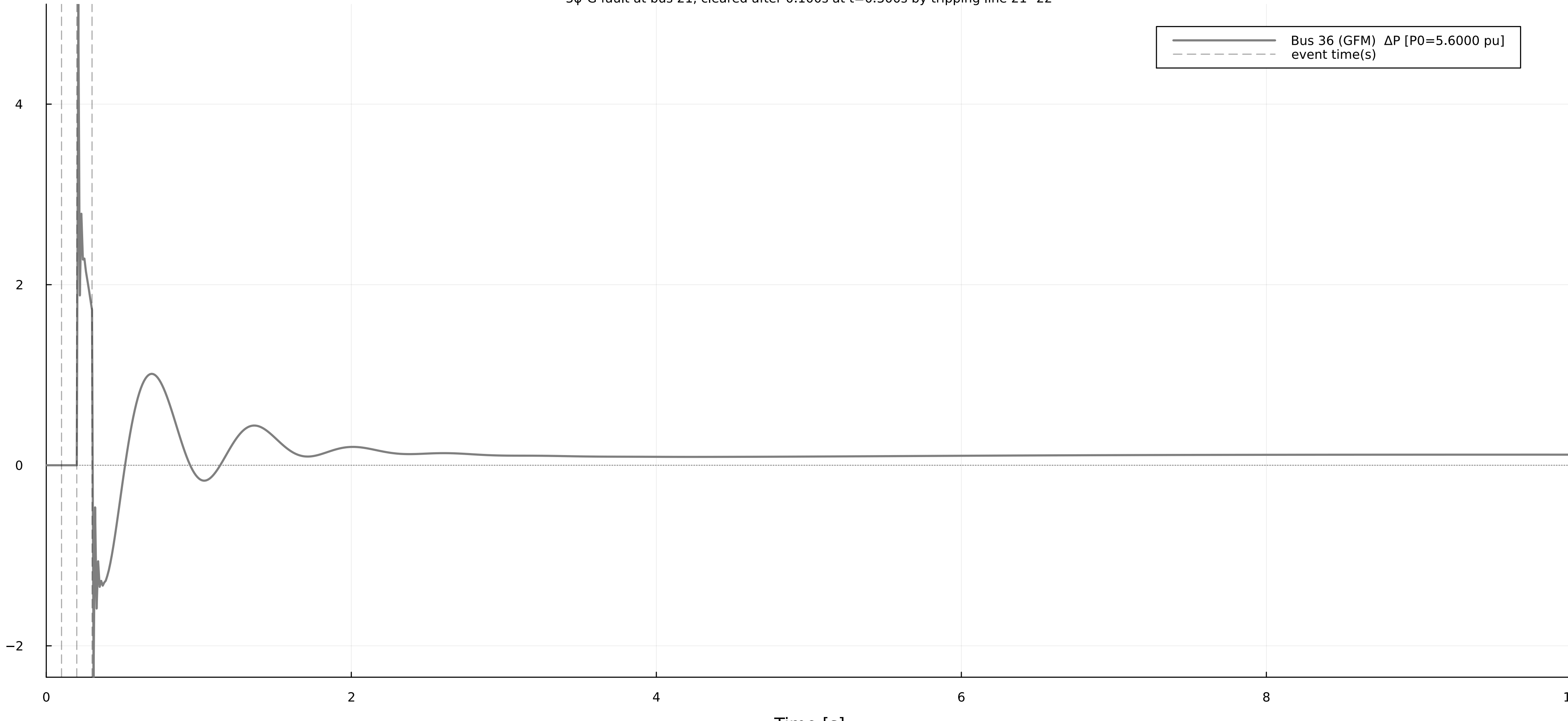
GFM active-power deviation at bus 36 3φ-G fault at bus 21, cleared after 0.100s at t=0.300s by tripping line 21--22
