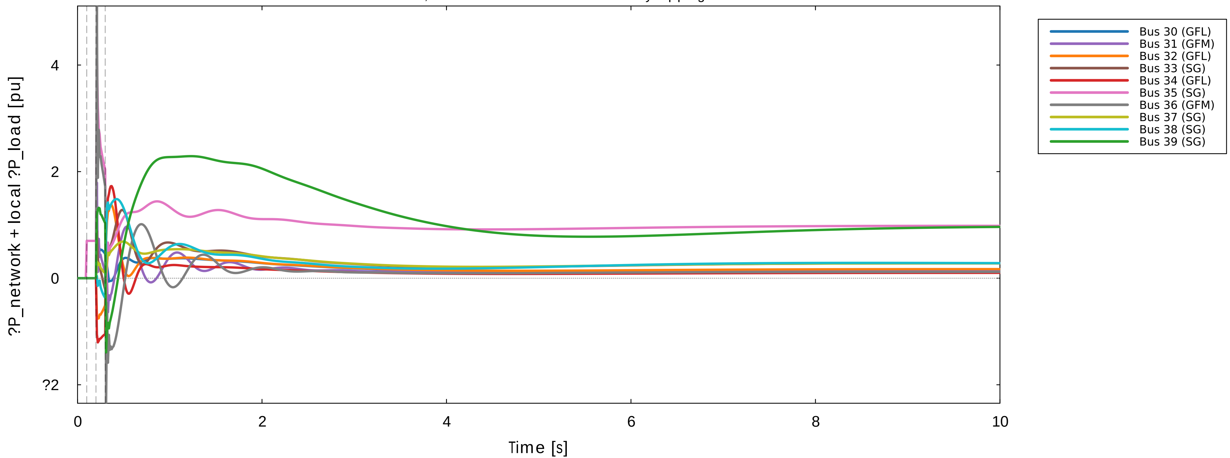
Reconstructed network active - power deviation from Ybus 3? - G fault at bus 21, cleared after 0.100s at t=0.300s by tripping line 21 - - 22
