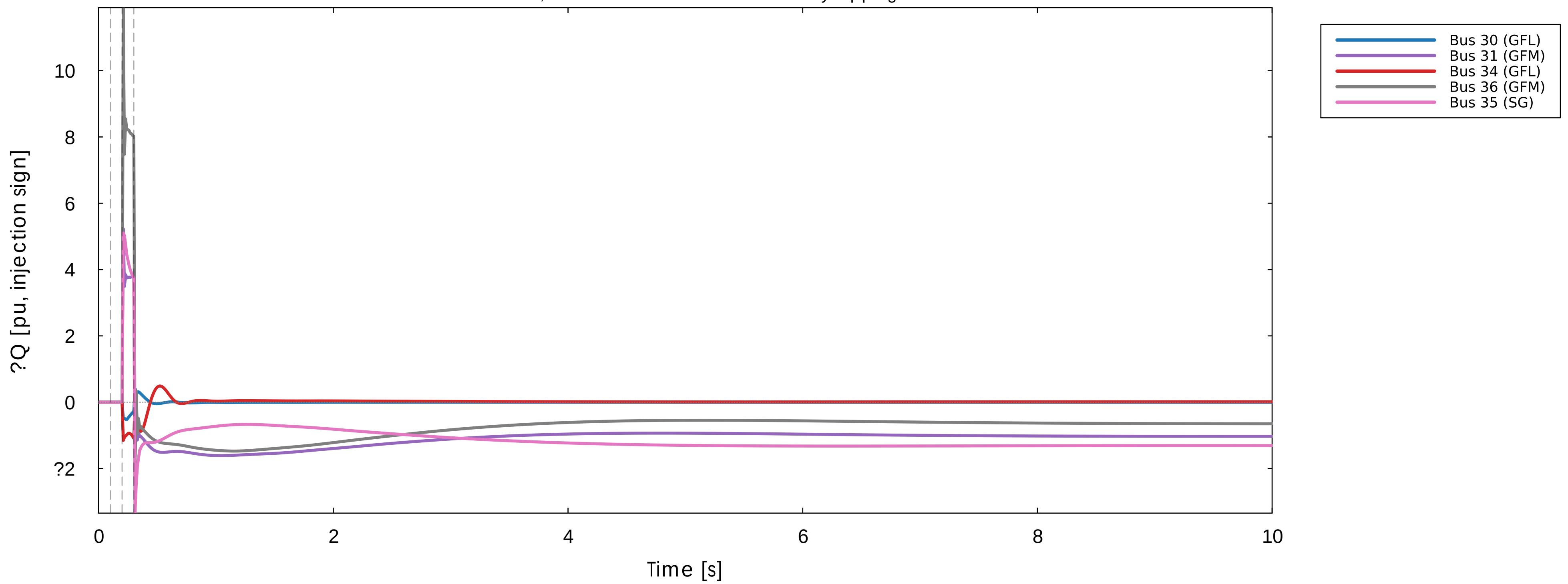
Terminal reactive - power deviation (device electrical output) 3? - G fault at bus 21, cleared after 0.100s at t=0.300s by tripping line 21 - - 22
