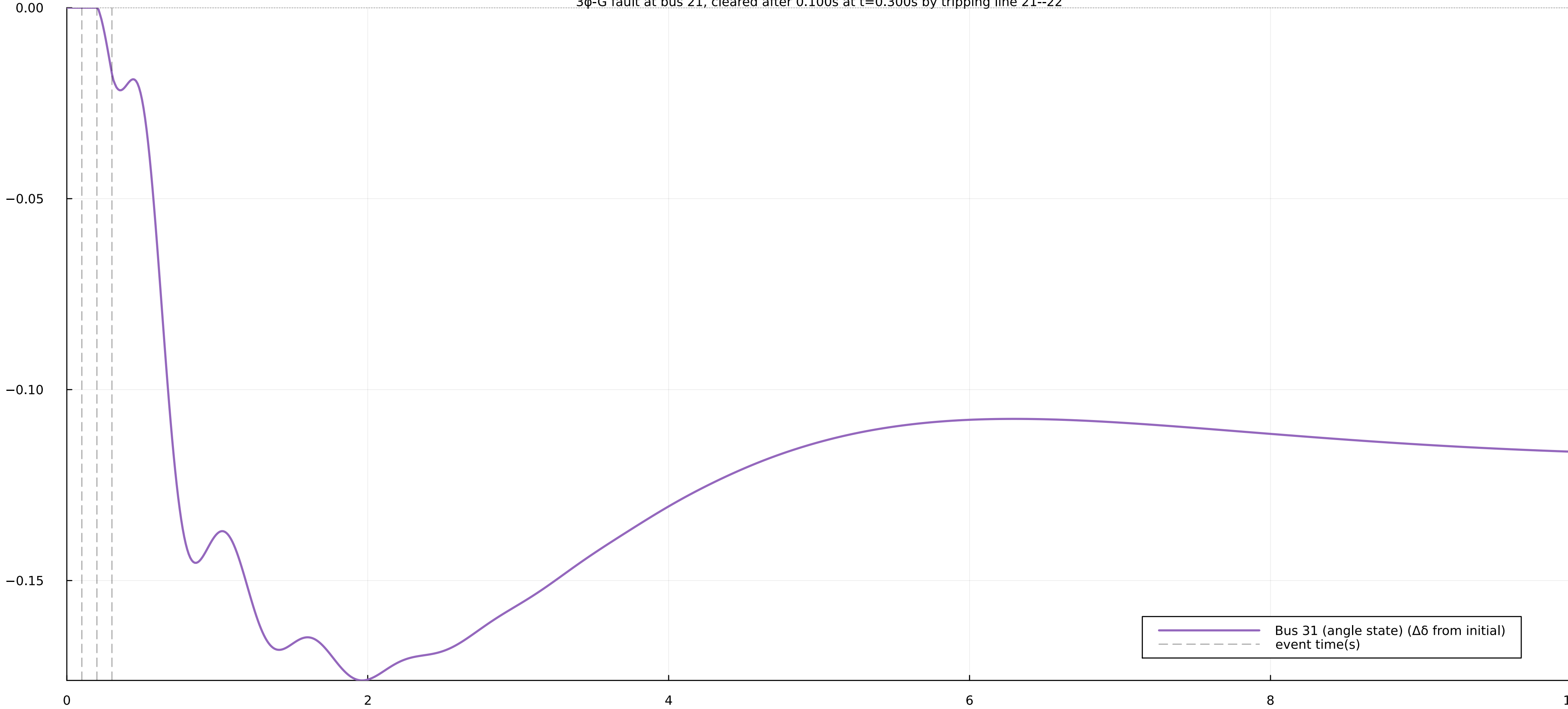
Rotor/angle deviation at bus 31 3 \phi -G fault at bus 21, cleared after 0.100s at t=0.300s by tripping line 21--22
